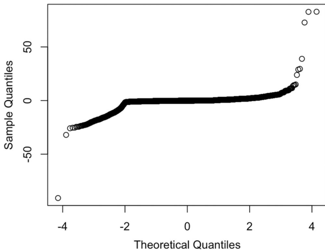
FIGURE A2 Normal Q-Q plot for top model.
